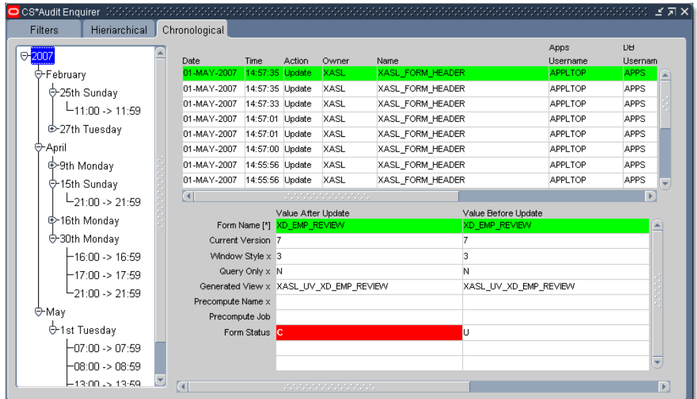
Figure2: Here we have the CS*Audit Enquirer in action. A simple to use but very powerful tool for querying audit data in a hierarchical and chronological format.
