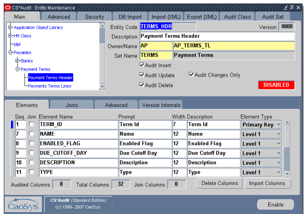
Figure 1: A screenshot of the CS*Audit Entity Maintenance screen in action.
