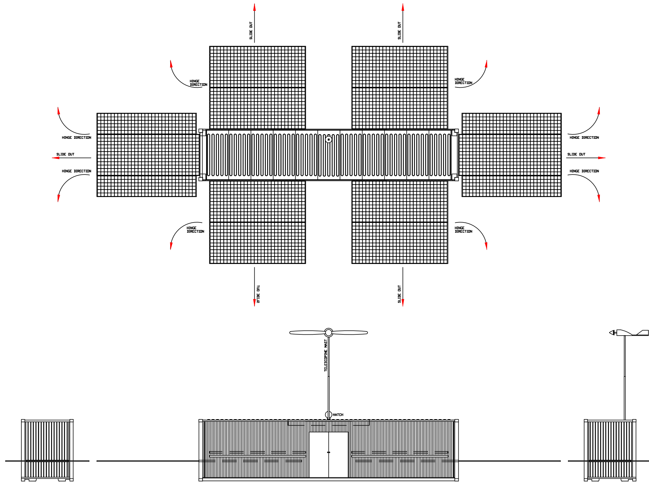
POWER ROOM CONTAINER = 8'-0 x 40'-0 x 8'-5 REMOTE HYBRID POWER STATION
