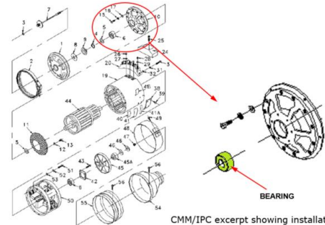
CMM/IPC excerpt showing installation of the Ball Bearing in the Starter-Generator
