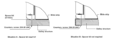
Installation of P/N 611053 Spacer Kit Assembly
