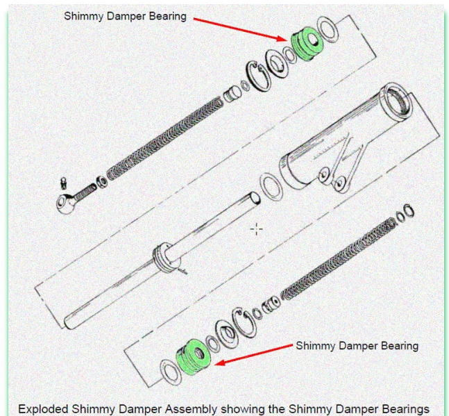
Exploded Shimmy Damper Assembly showing the Shimmy Damper Bearings
